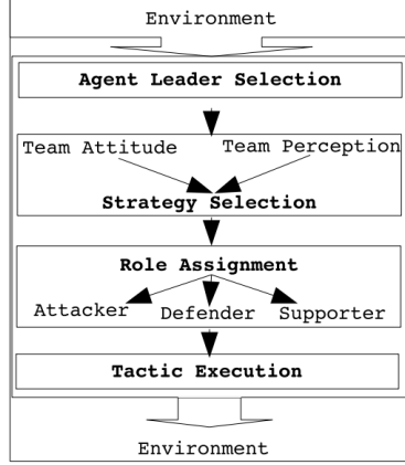
Fig. 7. Team Agent Behavior Architecture [5]
